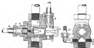
Figs. 2625-2626. Cut-out Cock for Engineer's Brake Valve, Atlantic (4-4-2) Locomotive, Pennsylvania R. R.
